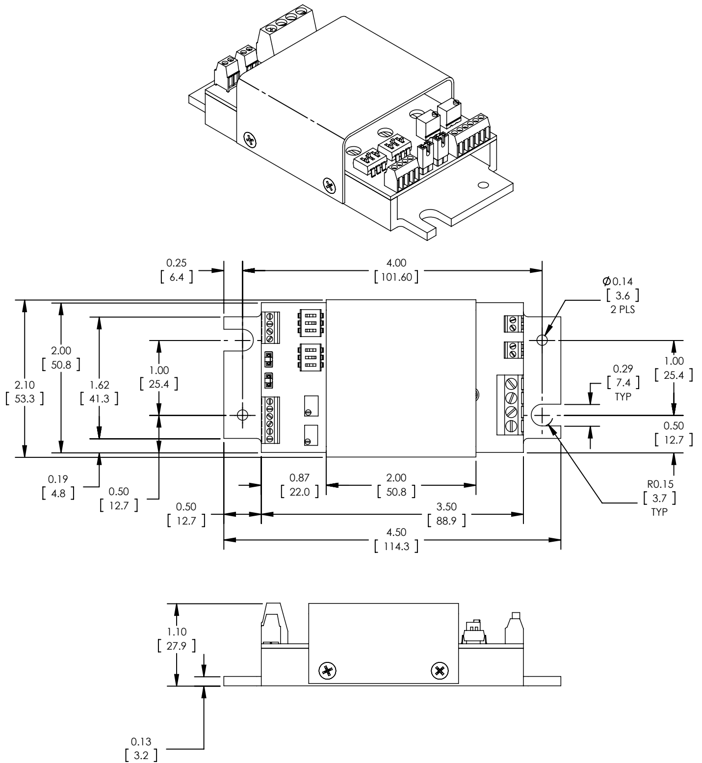
Figure 24. LDxCHA Driver Mechanical Dimensions
