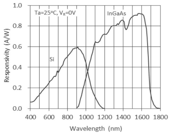
Spectral Responsivity
