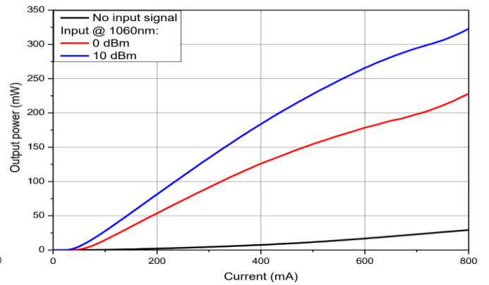
Output power at different input signals
