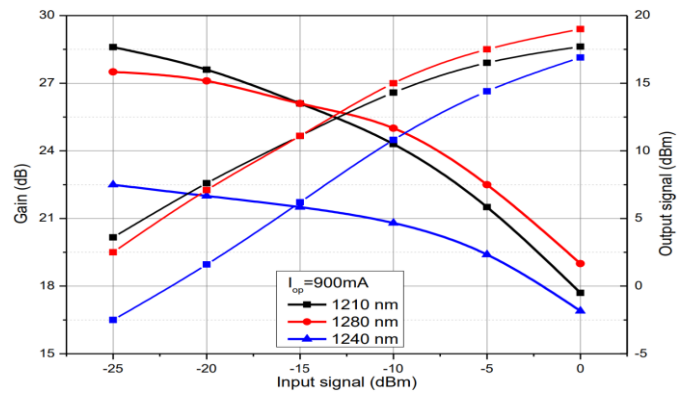
Gain and Output power vs. Input signal
