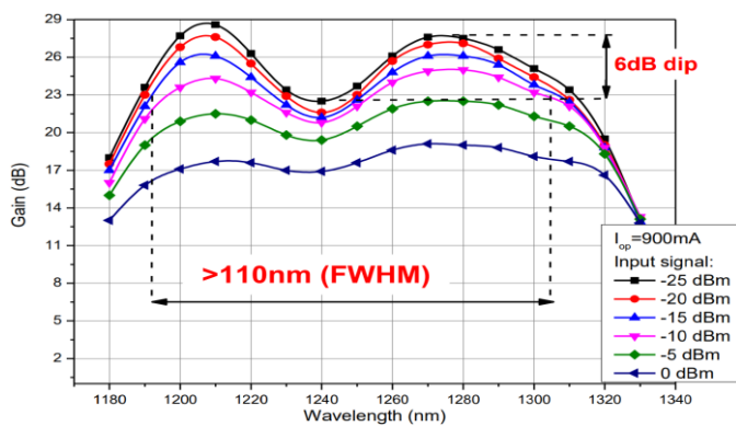
Gain spectra at different input signals
