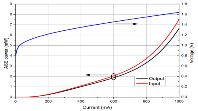
Output power at different input signals
