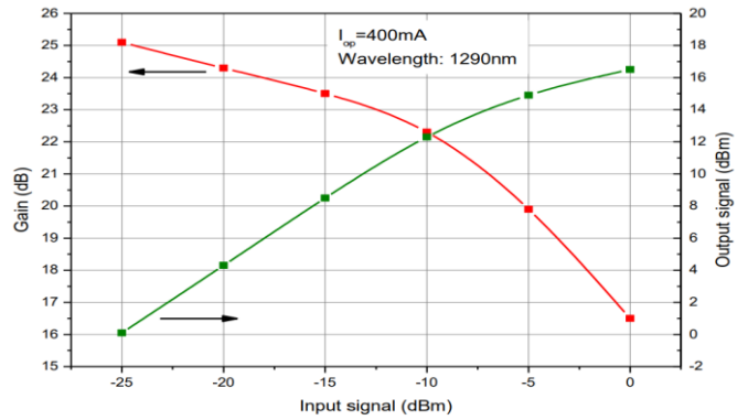
Gain and Output power vs. Input signal
