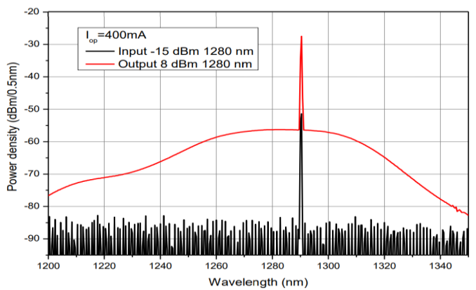
Spectra of amplified optical signal
