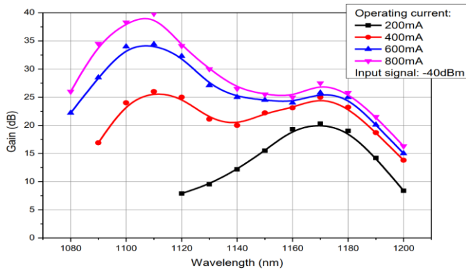
Gain spectra at different currents
