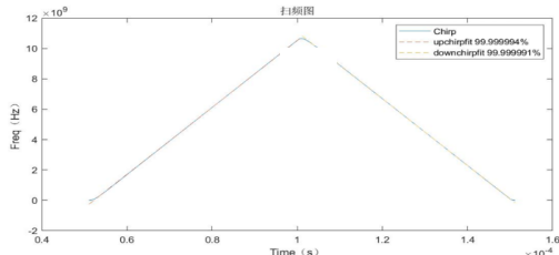
Measured Sweep Linearity: >> 99.9999%
